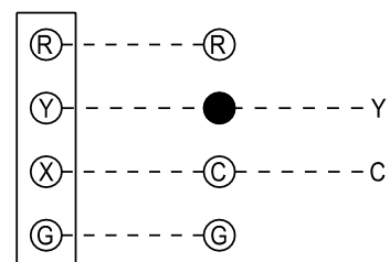
LOW VOLTAGE CONNECTION
