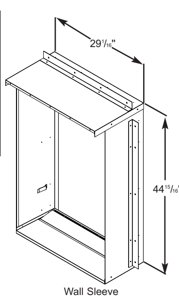
Wall Sleeve
