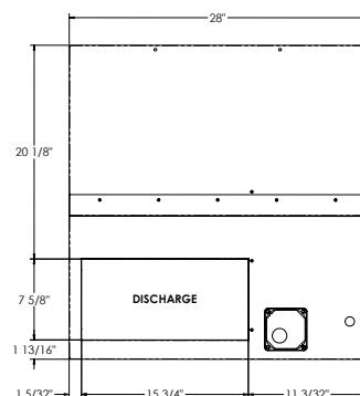
CPE Top View
